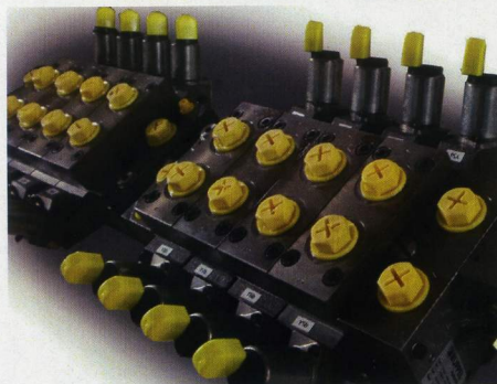
Figure 3: Valve blocks for the automated crane. Where necessary, the valves used by Ruppel Hydraulik were tailored to requirements, e.g. by using fully customised pistons.
