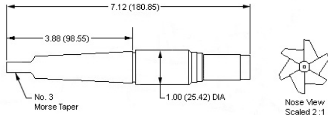
Dimensions shown are for reference only. in (mm)
