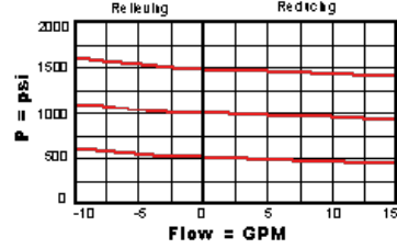
Regulated Pressure
