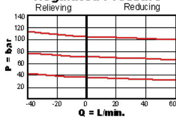
Regulated Pressure
